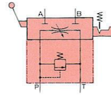
K FLOW CONTROL Friction detent
