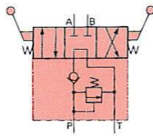
S SINGLE ACTING Spring centred
