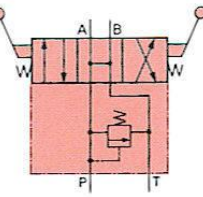
K FLOW CONTROL Friction detent
