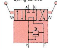
L DOUBLE ACTING HIGH FLOW Spring centred
